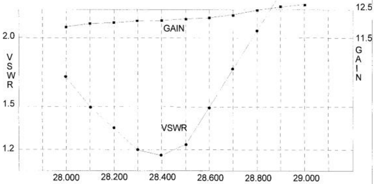
YP3-10M VSWR / GAIN CURVE
