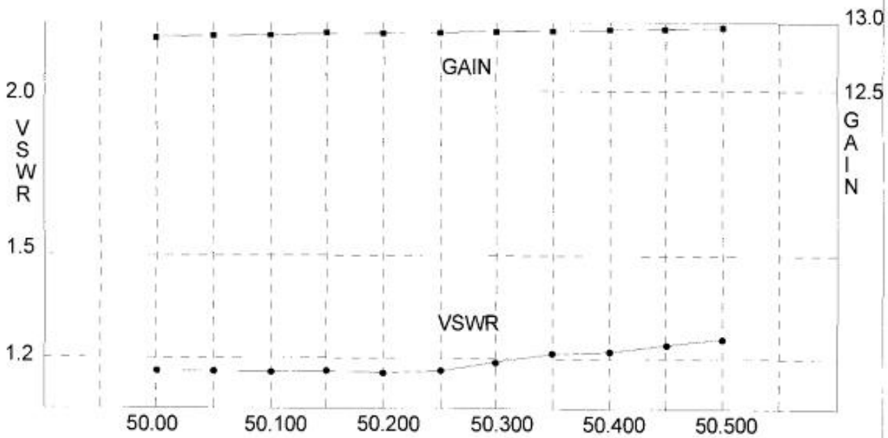
YP3-6M VSWR / GAIN CURVE
